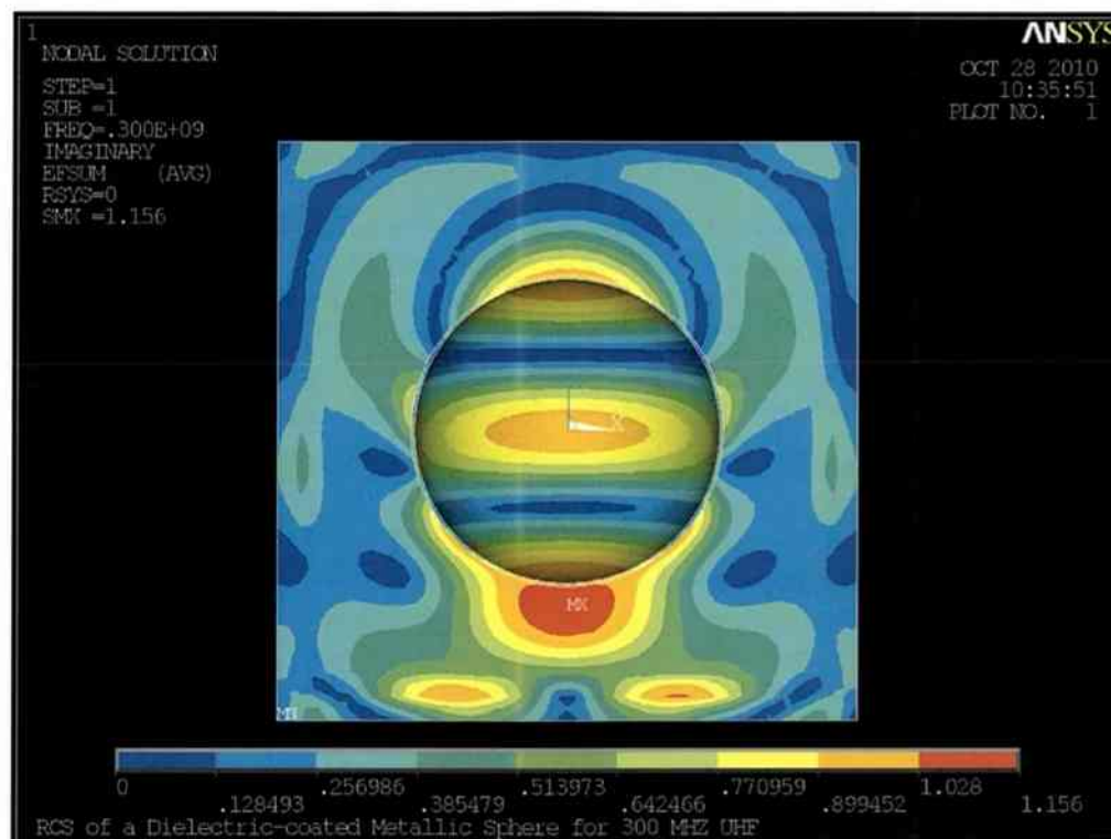
Figure 64. Electric Filed Contour in V/m for a 1/2 Symmetry 10 m Metallic Sphere with a 1 m Dielectric Coating in Decibels for 300 MHz and 25 Elements per Wavelength
